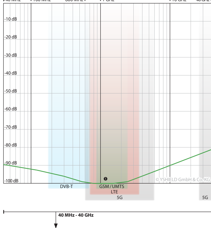
Screening attenuation Shielding netting HNG100 ● Single layer ● Double layer ● Three layer ▶40 MHz ▼100 MHz 600 MHz▼ ▼1 GHz ▼10 GHz 40 GHz◀
